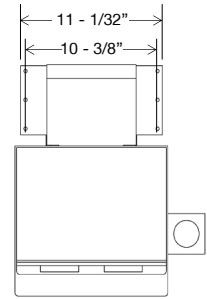
PLAN VIEW
